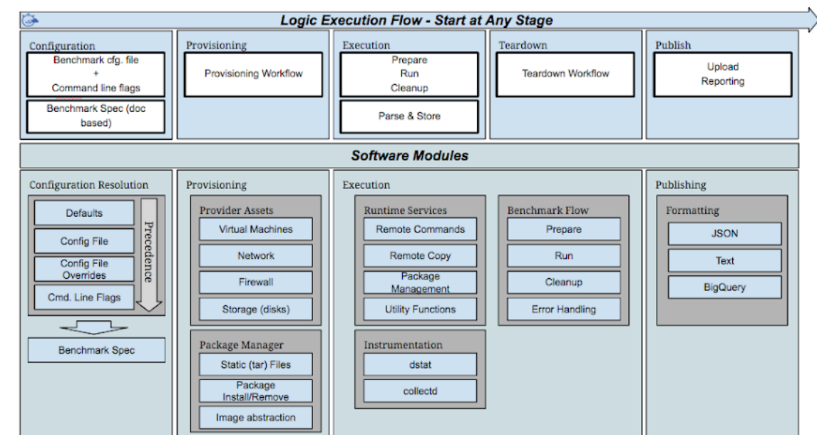
Fig. 1: PerfKit Benchmark Architecture Diagram
