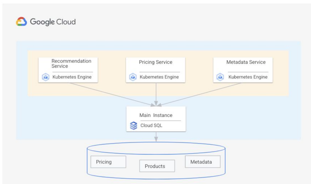
Microservices architecture
